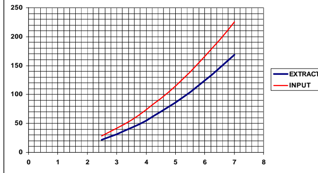
TYPICAL RESISTANCE WHEN USED AS TERMINAL ONLY SIZE 800
