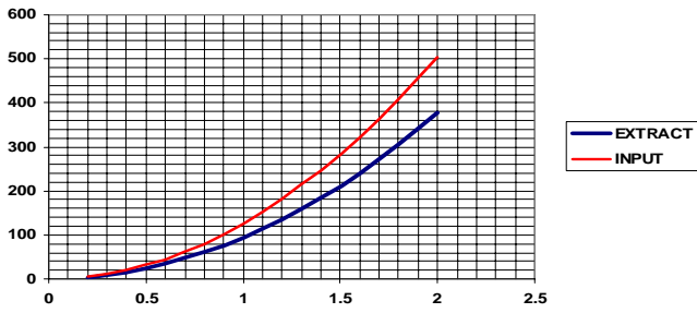
TYPICAL RESISTANCE WHEN USED AS TERMINAL ONLY SIZE 315/350
