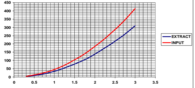
TYPICAL RESISTANCE WHEN USED AS TERMINAL ONLY SIZE 400/450
